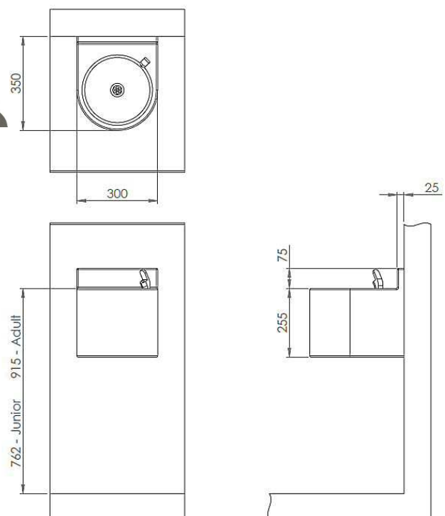
GWDF02 Drinking Fountain
